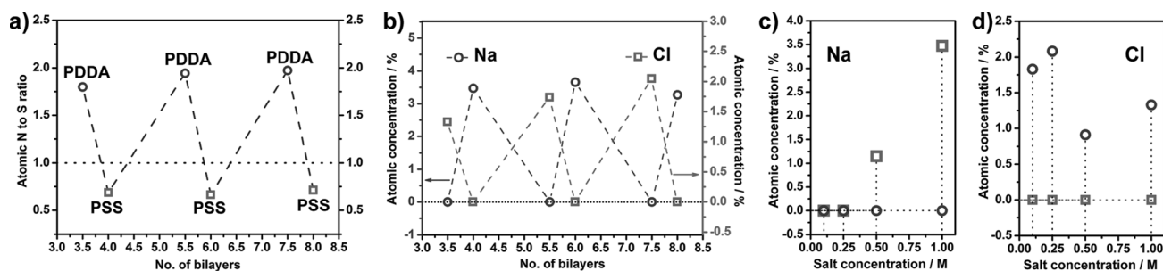
Figure 1. a) Plot of the N to S atomic ratios on (PDDA/PSS) n PEMs, prepared by LbL deposition in 1.0 M NaCl, versus the bilayer number. b) Plot of the atomic concentration of Na (circles) and Cl (squares) on (PDDA/PSS) n PEMs, prepared by LbL deposition in 1.0 M NaCl, versus the bilayer number. Plot of the atomic concentration of Na (c) and Cl (d) on PDDA- (circles) and PSS-capped (squares) surfaces versus the NaCl concentration used for LbL growth of (PDDA/PSS) n PEMs. In Figure c and d, (PDDA/PSS) 3.5 and (PDDA/PSS) 4.0 PEMs, obtained in 1.0 M NaCl, are compared with the PDDA-capped and PSS-capped PEMs, obtained in dilute NaCl, with similar thickness and roughness. [9] All the data are obtained from XPS measurements.
